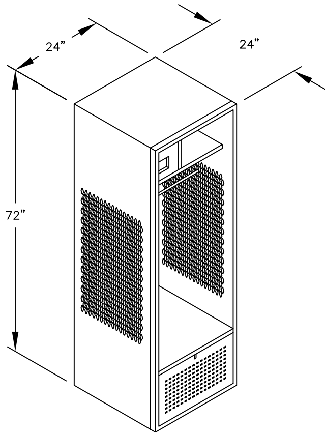
MODEL #70024 24" WIDE OPEN ACCESS STANDARD LOCKER
