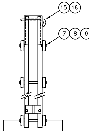
(CARRIAGE ASSEMBLY)
